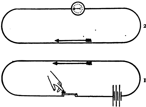
FIG. 426.—Diagram Illustrating the Action of Voltaic Induction Between Two Circuits: the one including a source of electrical energy and a switch; the other including a galvanometer, but having no cell or other electrical source. The direction of the battery current in circuit 1 is indicated by the arrow; the arrow in circuit 2 showing the direction of the induced current.
